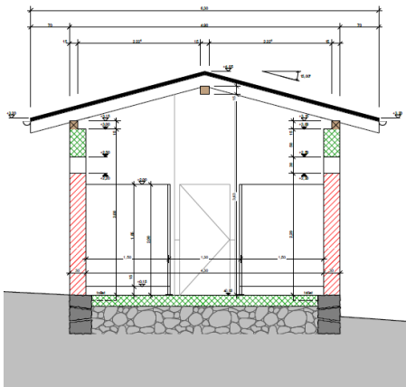
cut A
