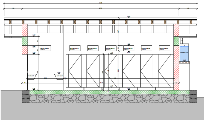
cut B
